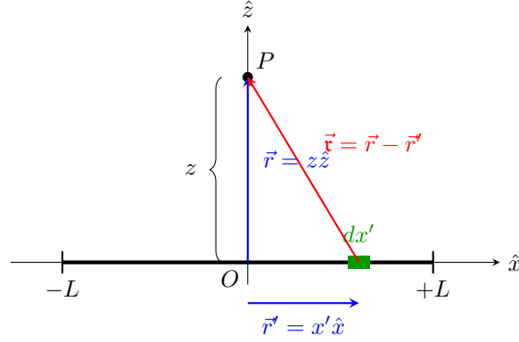
Figure 2: Setup for the finite line of charge. The source point \vec{r}' = x'\hat{x} runs from -L to L ; the field point is P at \vec{r} = z\hat{z} ; the separation vector is \vec{r} = \vec{r} - \vec{r}' .
